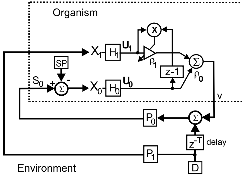
Figure 2: ICO learning embedded into its environment. \Sigma is a linear summation unit. Except for the constant set-point SP , the inside of the organism resembles ICO learning as shown in Fig. 1 A, but here shown without the filter bank and transformed into the z -domain. D is a disturbance which is delayed by T time-steps. The term z-1 denotes a derivative in the z -domain. Transfer functions P_0 and P_1 represent the environment and establish the feedback from the motor output v to the sensor inputs x_0 and x_1 . S_0 represents the input before subtracting the setpoint.
