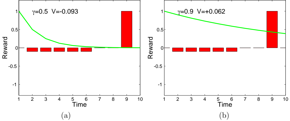
Fig. 7. The effect of discount factor \gamma in decision making. In a scenario where negative reward (cost) is expected before achieving a large positive reward, the cumulative future reward V becomes negative if \gamma is small (a) and positive if \gamma is large enough (b). Assuming that there is a baseline behavior where the expected reward is zero, such behavior is rejected as negligible with a small \gamma .
