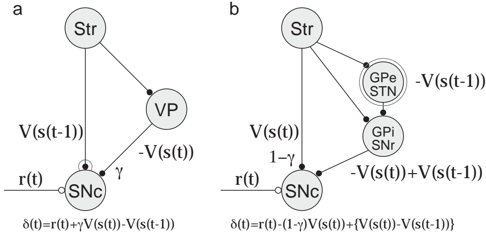
Fig. 6. Possible mechanisms for temporal difference computation of the value function represented in the basal ganglia. The circles \circ represent excitatory connection while black dots \bullet represents inhibitory connections. A large gray circle represents a source of possible time delay. SNc and SNr: compact and reticular parts of substantia nigra. Str: striatum. GPi and GPe: internal and external segments of globus pallidus. STN: subthalamic nucleus.
