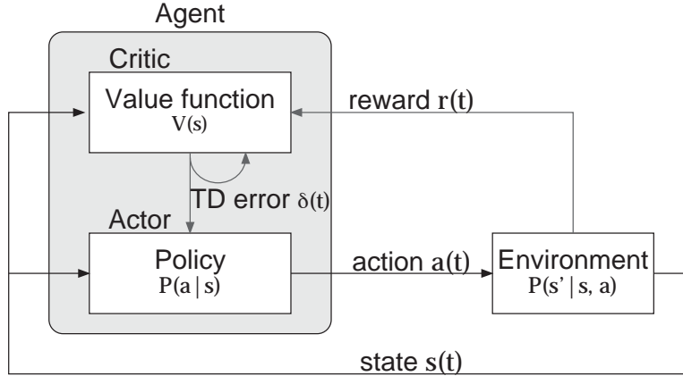
Fig. 2. A standard architecture for reinforcement learning, known as actor-critic . The agent has a two-part organization: the critic learns the state value function V(s) and the actor learns the policy P(a|s) . The temporal difference (TD) error \delta(t) is used as the error signal for the learning of the critic and the reinforcement signal is used for the learning of the actor.
